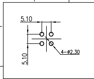
4 Pin PCB Layout
