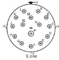
Contact Layout
