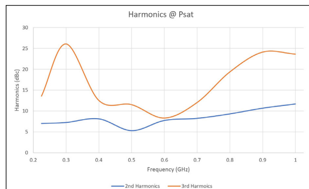
Harmonics @ Psat
