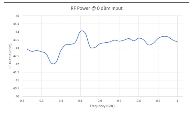
RF Output Power @ 0 dBm Input
