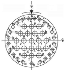
Contact Layout
