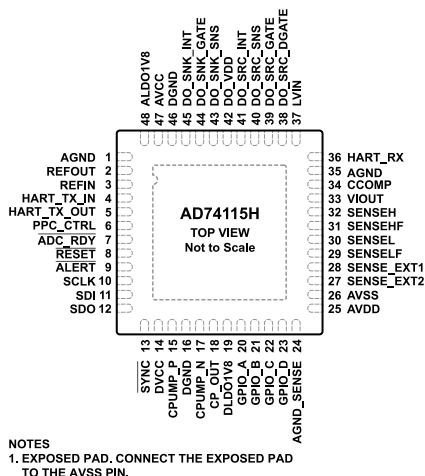
Figure 4. Pin Configuration
