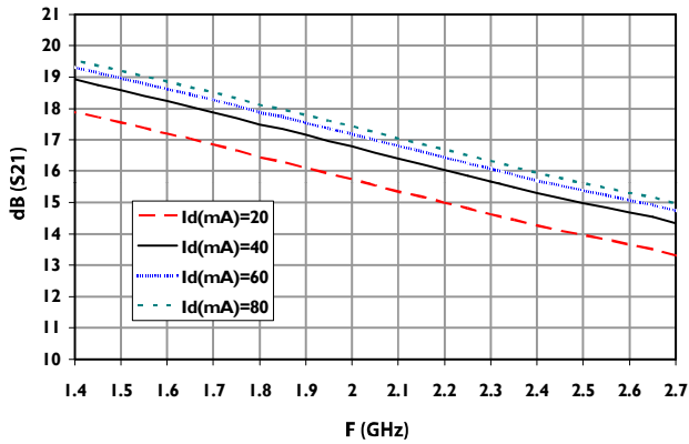
Gain
