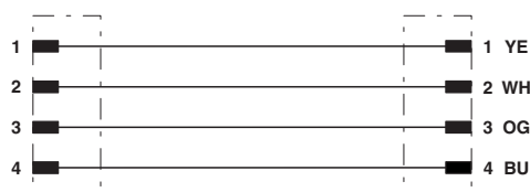
Contact assignment of the M12 plugs
