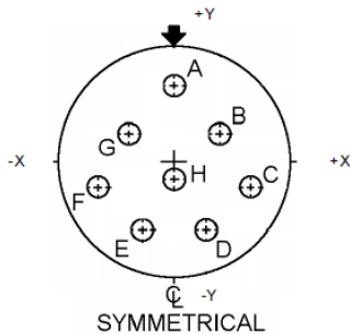
Contact Layout
