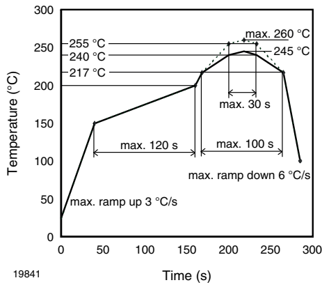
Fig. 10 - Lead (Pb)-free Reflow Solder Profile According to J-STD-020
